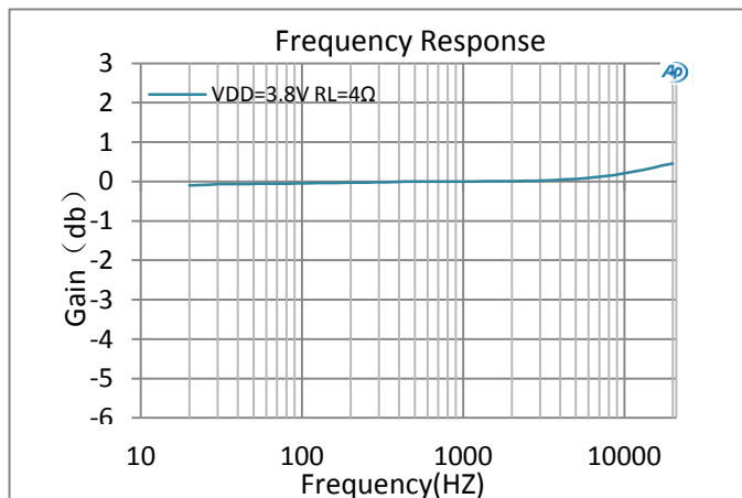
图5: Frequency Response
