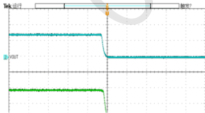
Overdischarge Protection OCP +
