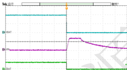
Battery Charging, OCP
