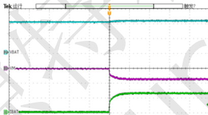
Battery Charging OVP
