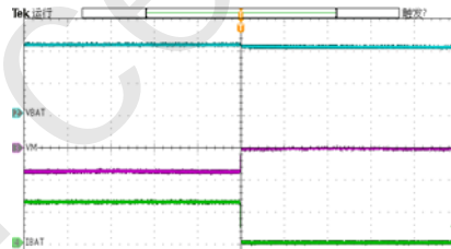
Overdischarge Protection UVP
