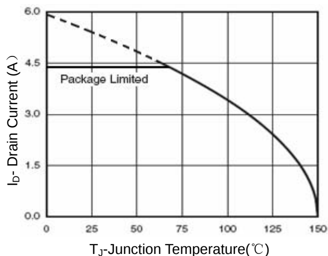
Figure 4 Drain Current
