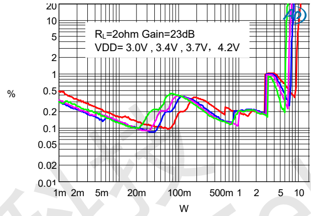
THD+N vs Output Power_2Ω
