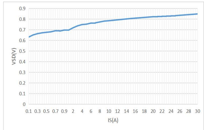
Figure 6: Body-Diode Characteristics
