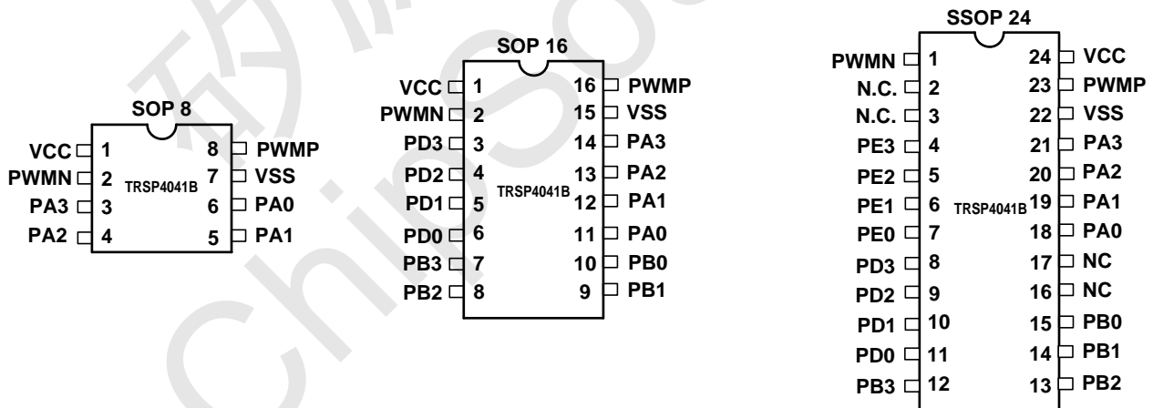
Figure1. Package definition
