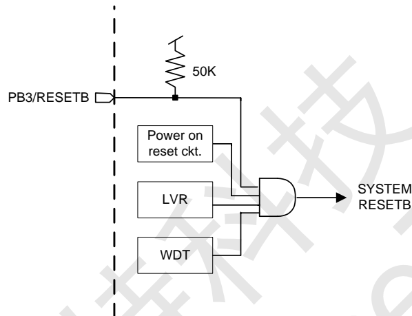
Figure 4 Reset structure
