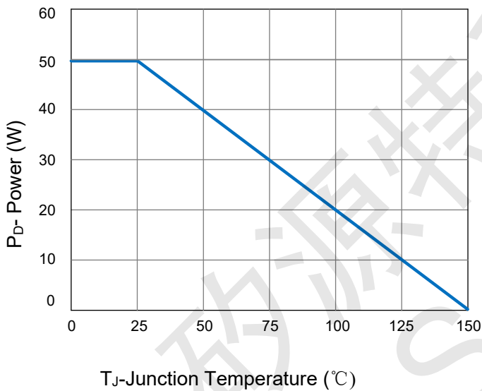
Figure 3 Power De-rating
