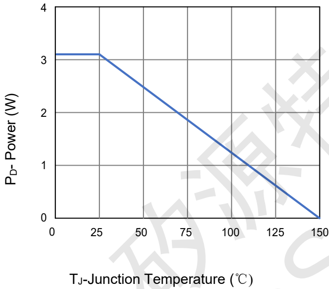
Figure 3 Power De-rating
