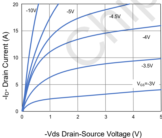
Figure 5 Output Characteristics
