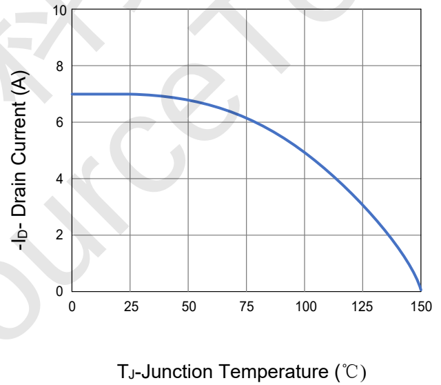
Figure 4 Drain Current
