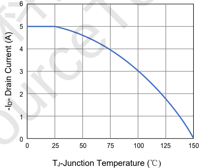
Figure 4 Drain Current
