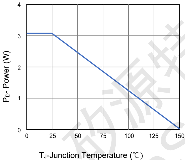
Figure 3 Power De-rating
