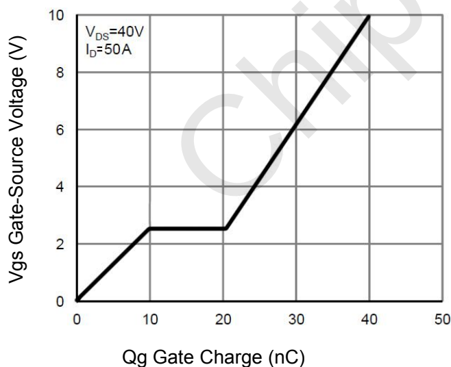
Figure 11 Gate Charge
