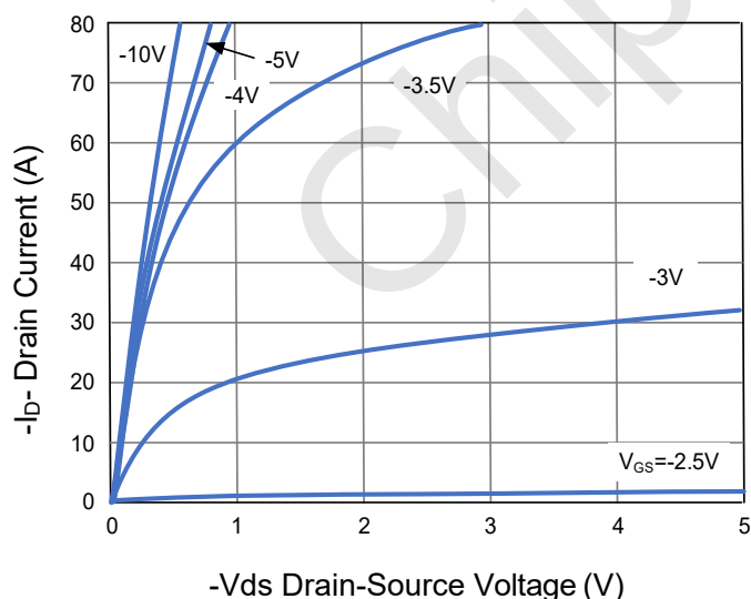
Figure 5 Output Characteristics
