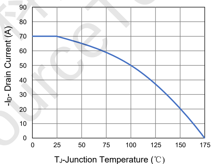
Figure 4 Drain Current
