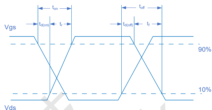
Figure 2 Switching Waveform
