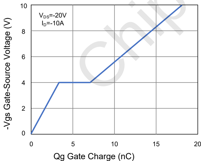
Figure 11 Gate Charge
