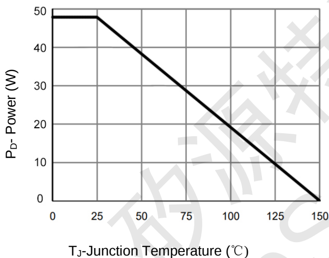
Figure 3 Power De-rating
