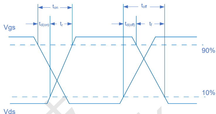
Figure 2 Switching Waveform
