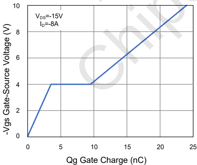
Figure 11 Gate Charge
