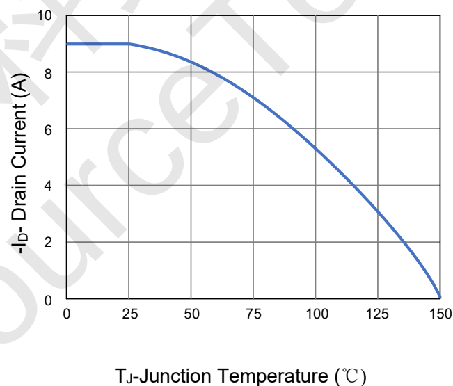
Figure 4 Drain Current
