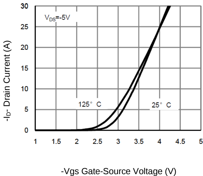
Figure 7 Transfer Characteristics
