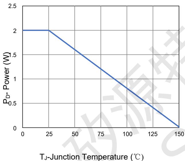
Figure 3 Power De-rating
