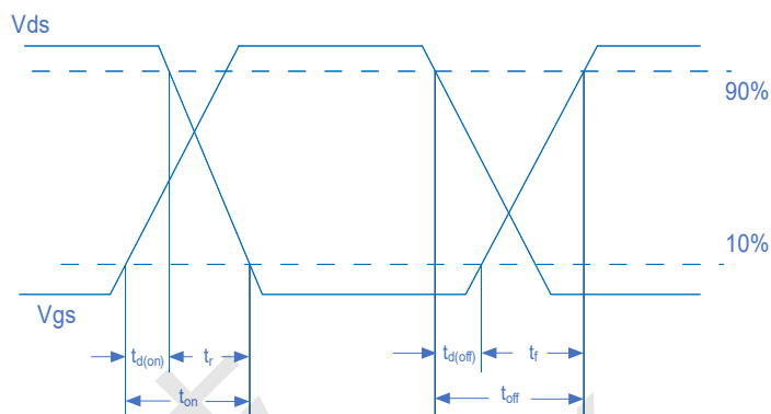
Figure 2 Switching Waveform
