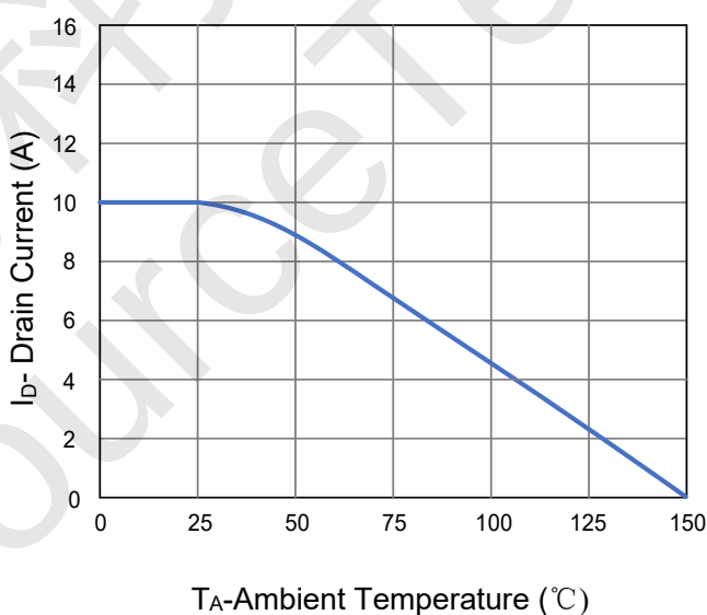
Figure 4 Drain Current
