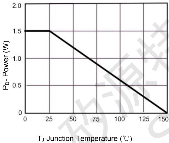
Figure 3 Power Dissipation
