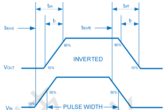
Figure 2 Switching Waveform
