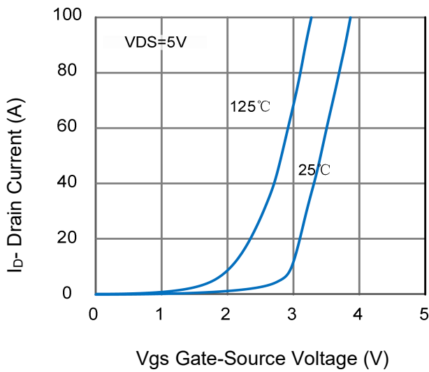
Figure 7 Transfer Characteristics
