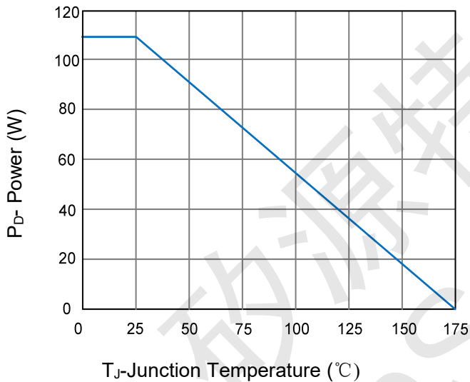
Figure 3 Power De-rating
