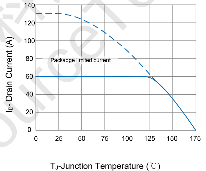
Figure 4 Drain Current
