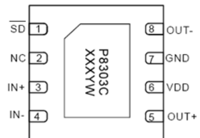
U-DFN3030-8 (C)
