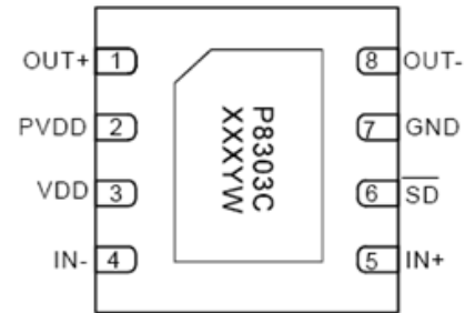
U-DFN3030-8 (B)
