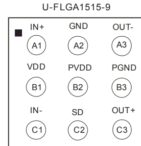
PAM8013
