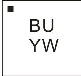
PAM8013- U-FLGA1515-9
