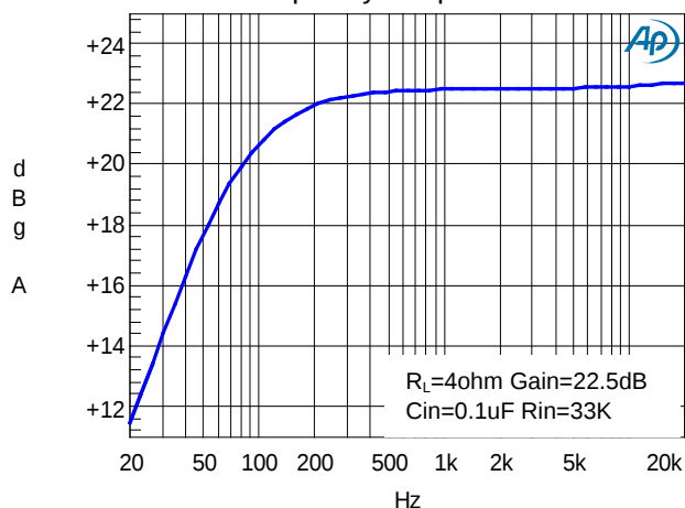
Frequency Response
