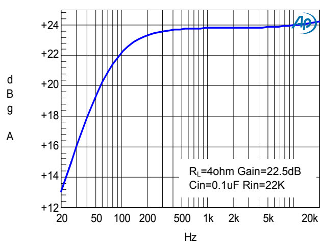
Frequency Response
