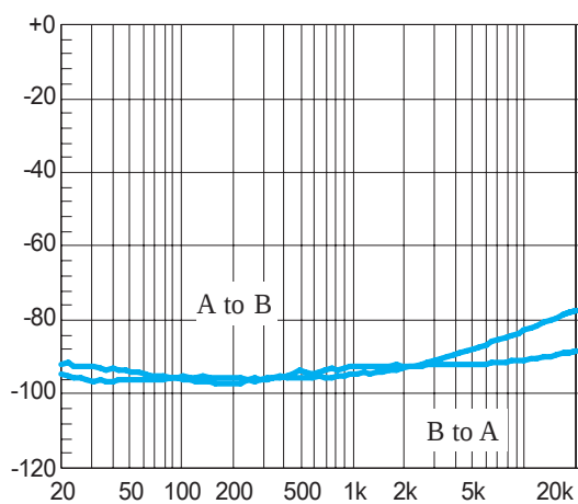
Figure 27. Crosstalk BTL mode, 6V, 8Ohm, P_o=1W
