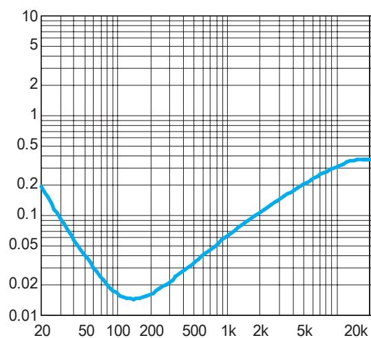
Figure 10. THD+N vs. Frequency BTL mode, 3V, 80hm, P_o=300\text{mW}
