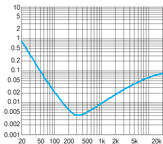
Figure 11. THD+N vs. Frequency SE mode, 6V, 320hm, P_o=70\text{mW}
