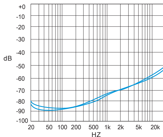
Figure 18. PSRR vs. Freq BTL mode, 3V, 80hm, 200mVpp Input unterminated
