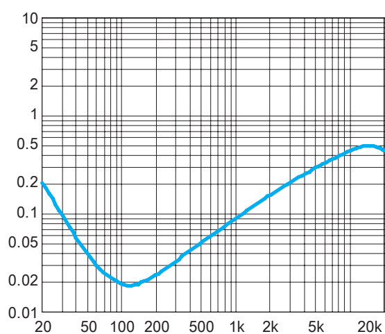
Figure 14. THD+N vs. Frequency BTL mode, 3V, 40hm, P_o=500\text{mW}
