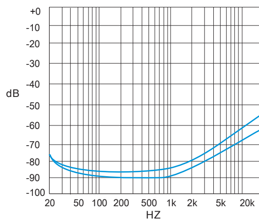
Figure 20. PSRR vs. Freq SE mode, 3V, 320hm, 200mVpp Input terminated
