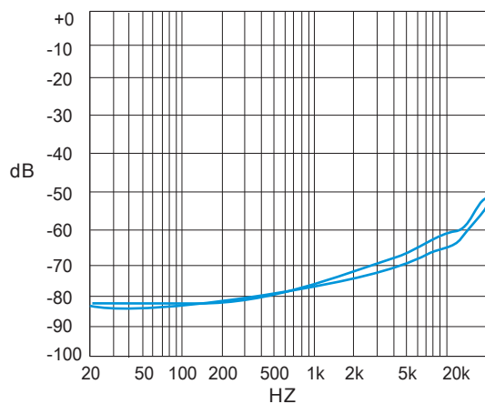
Figure 15. PSRR vs. Freq BTL mode, 6V, 80hm, 200mVpp Input terminated
