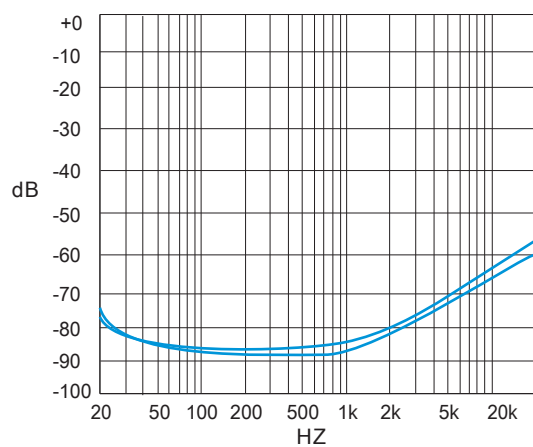
Figure 19. PSRR vs. Freq SE mode, 6V, 320hm, 200mVpp Input terminated
