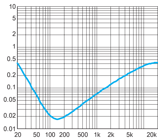
Figure 13. THD+N vs. Frequency BTL mode, 6V, 40hm, P_o=1\text{W}
