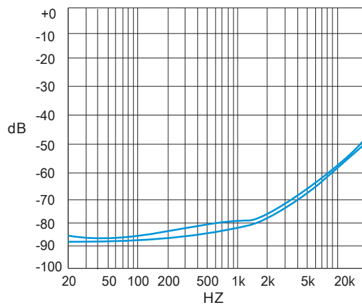
Figure 16. PSRR vs. Freq BTL mode, 3V, 80hm, 200mVpp Input terminated
