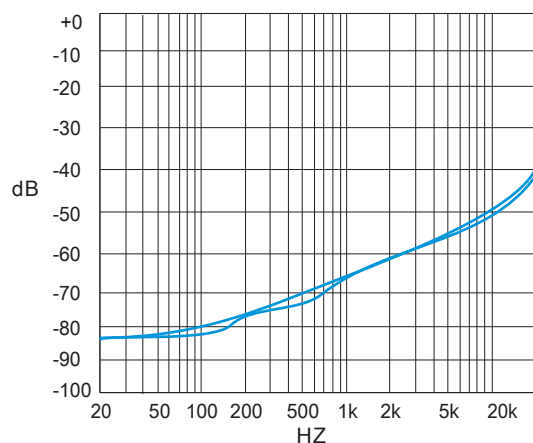
Figure 17. PSRR vs. Freq BTL mode, 6V, 80hm, 200mVpp Input unterminated
