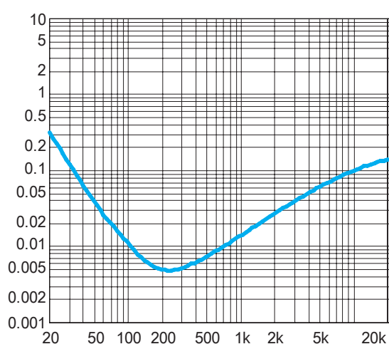
Figure 12. THD+N vs. Frequency SE mode, 3V, 320hm, P_o=20\text{mW}
