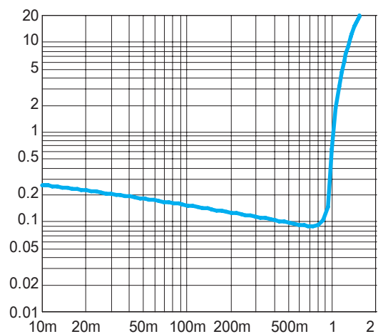
Figure 8. THD+N vs. Output Power BTL mode, 3V, 4Ohm, f=1 kHz
