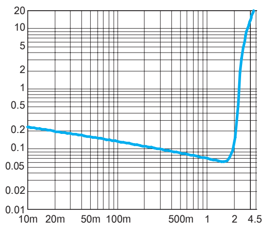
Figure 7. THD+N vs. Output Power BTL mode, 6V, 4Ohm, f=1 kHz
