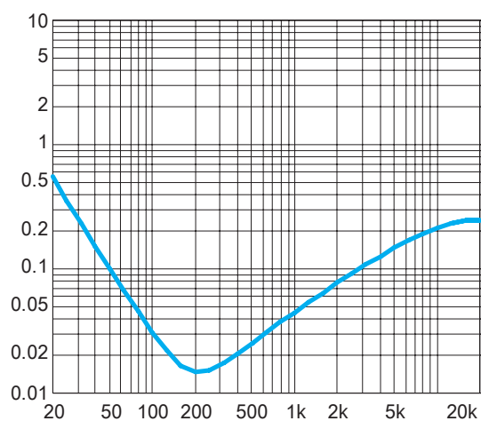
Figure 9. THD+N vs. Frequency BTL mode, 6V, 80hm, P_o=800\text{mW}
