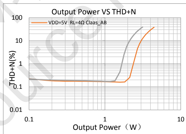
图 4. Output Power VS THD+N
