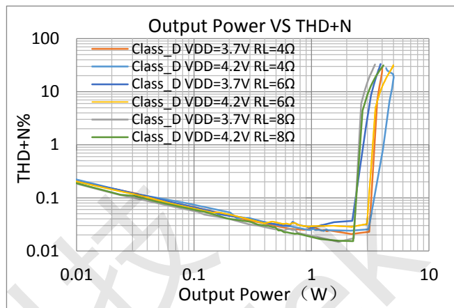
图2. Output Power VS THD+N
