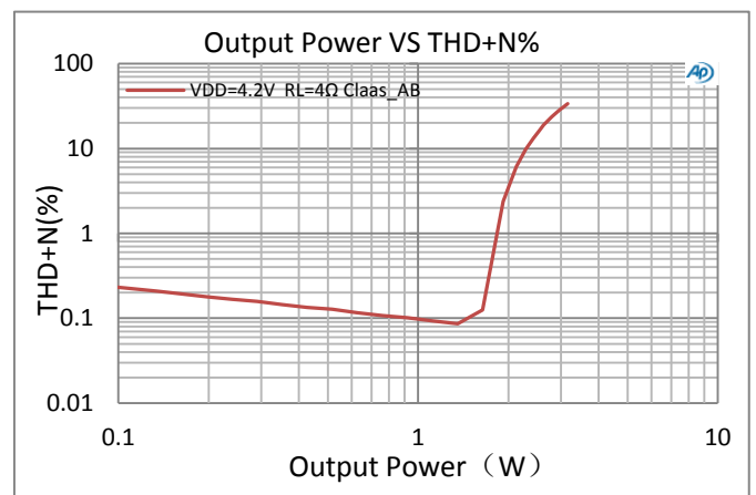
图4: THD+N VS. Output Power Class_AB
