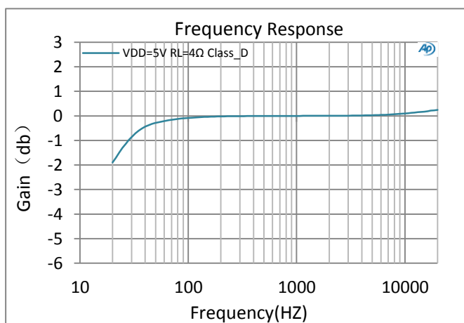
图8: Frequency Response
