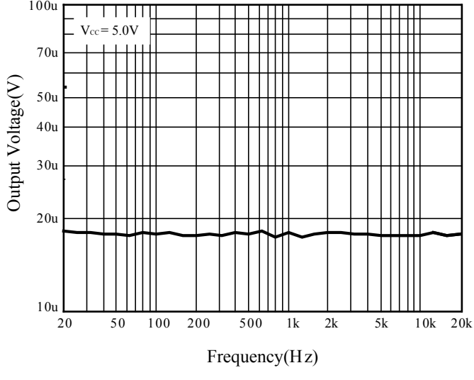
Figure 7 Noise Floor
