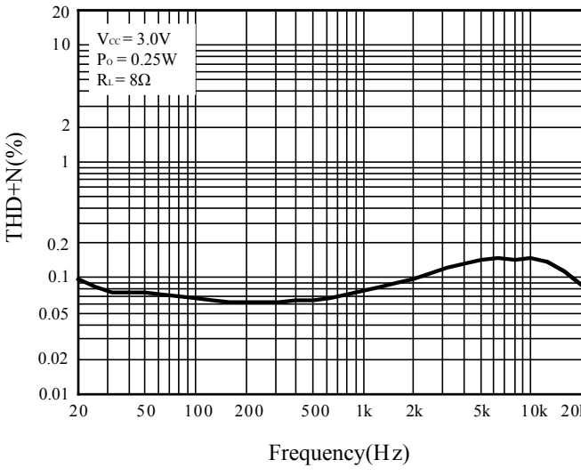
Figure 4 THD+N vs. Frequency
