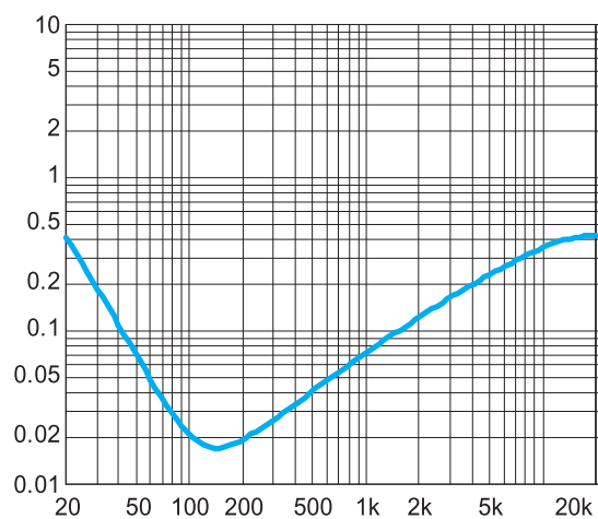
Figure 13. THD+N vs. Frequency BTL mode, 6V, 40Ω, P_o=1\text{W}
