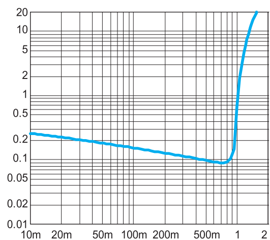
Figure 8. THD+N vs. Output Power BTL mode, 3V, 40Ω, f=1 kHz
