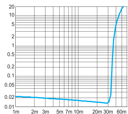
Figure 6. THD+N vs. Output Power SE mode, 3V, 320Ω, f=1 kHz
