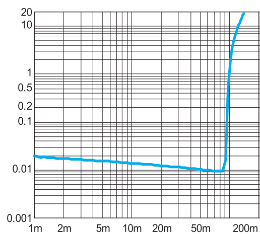
Figure 5. THD+N vs. Output Power SE mode, 5V, 320Ω, f=1 kHz
