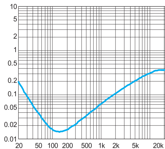
Figure 10. THD+N vs. Frequency BTL mode, 3V, 80Ω, P_o=300\text{mW}
