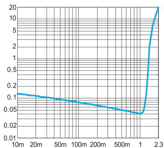
Figure 3. THD+N vs. Output Power 6V, 80Ω, BTL at f=1 kHz
