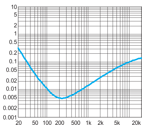
Figure 12. THD+N vs. Frequency SE mode, 3V, 320Ω, P_o=20\text{mW}
