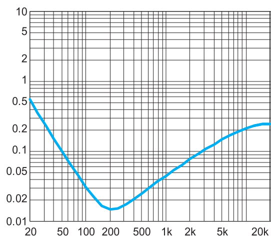
Figure 9. THD+N vs. Frequency BTL mode, 6V, 80Ω, P_o=800\text{mW}
