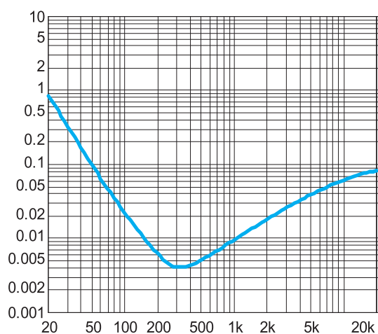
Figure 11. THD+N vs. Frequency SE mode, 6V, 320Ω, P_o=70\text{mW}
