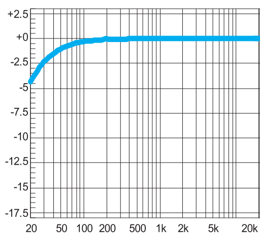
Figure 25. Frequency Response SE mode, 6V, 320hmC5/C6=220uF
