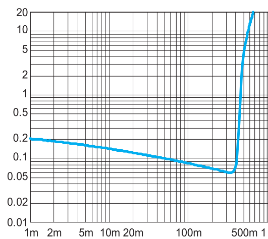
Figure 4. THD+N vs. Output Power 3V, 80Ω, BTL at f=1 kHz
