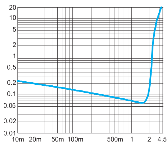
Figure 7. THD+N vs. Output Power BTL mode, 6V, 40Ω, f=1 kHz
