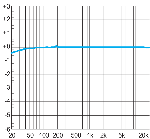
Figure 23. Frequency Response BTL mode, 6V, 80hm
