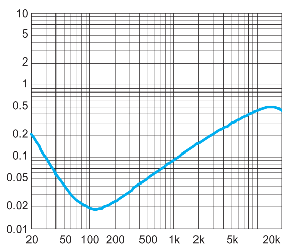
Figure 14. THD+N vs. Frequency BTL mode, 3V, 40Ω, P_o=500\text{mW}
