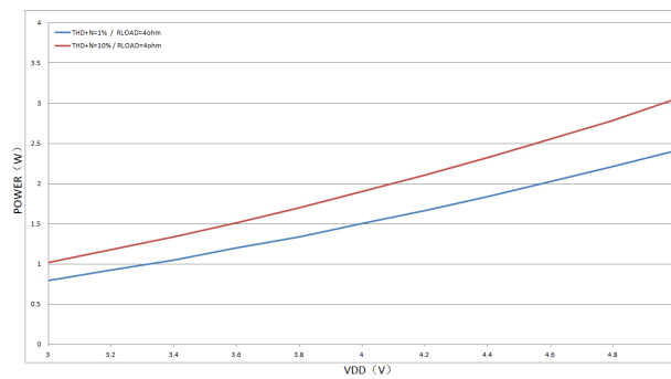
VDD VS. Power
